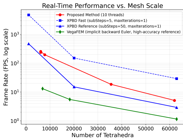
FIGURE 7. Frame rate versus mesh scale (log-scale FPS axis) for the proposed method (10 threads), XPBD under the Fast and Reference substep configurations defined in Section IV-A, and VegaFEM. The proposed method maintains better real-time performance than VegaFEM over a broad tetrahedral range and still retains basic interactivity on larger-scale models.
